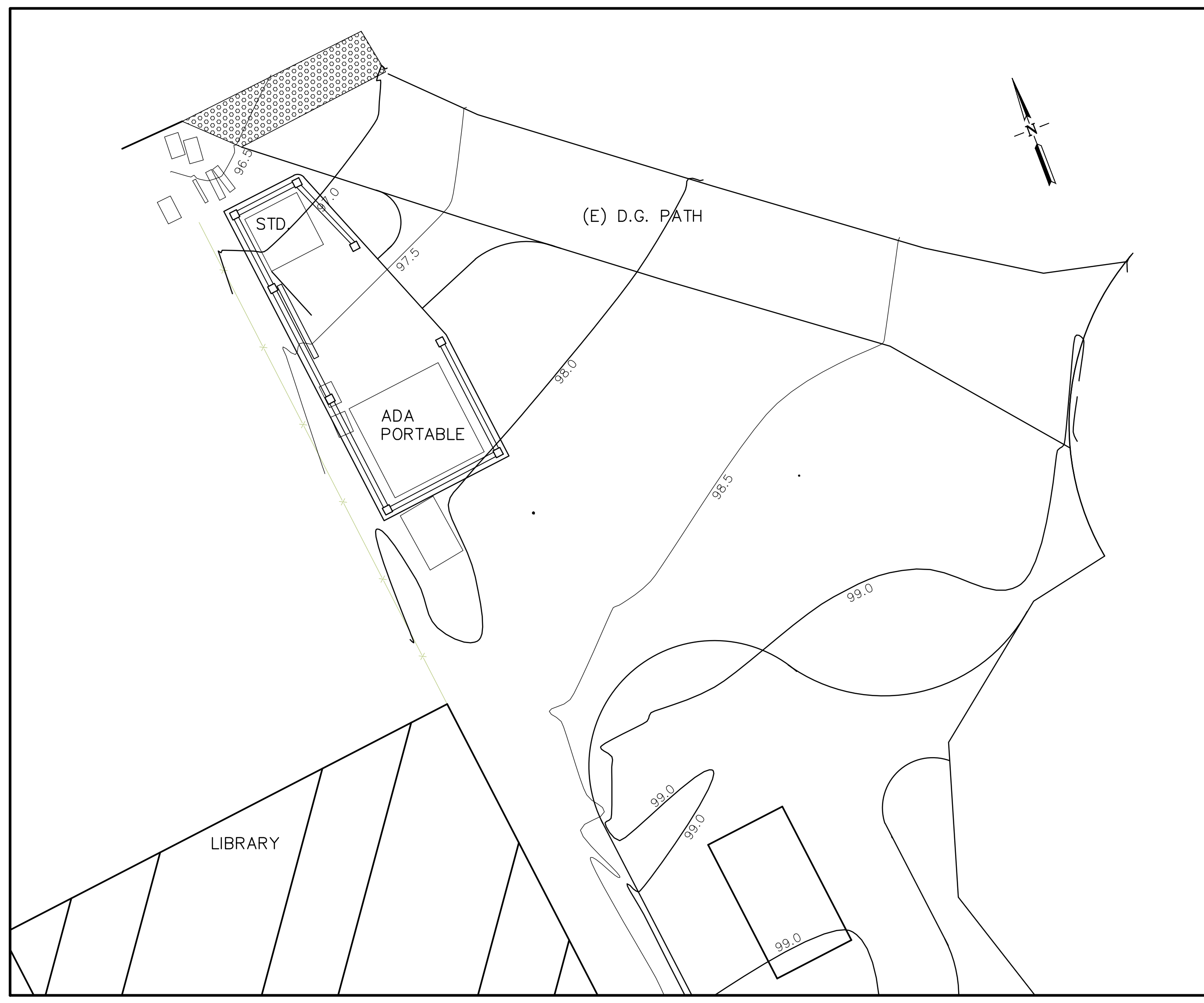
GRADING PLAN 1"=5'-0"
