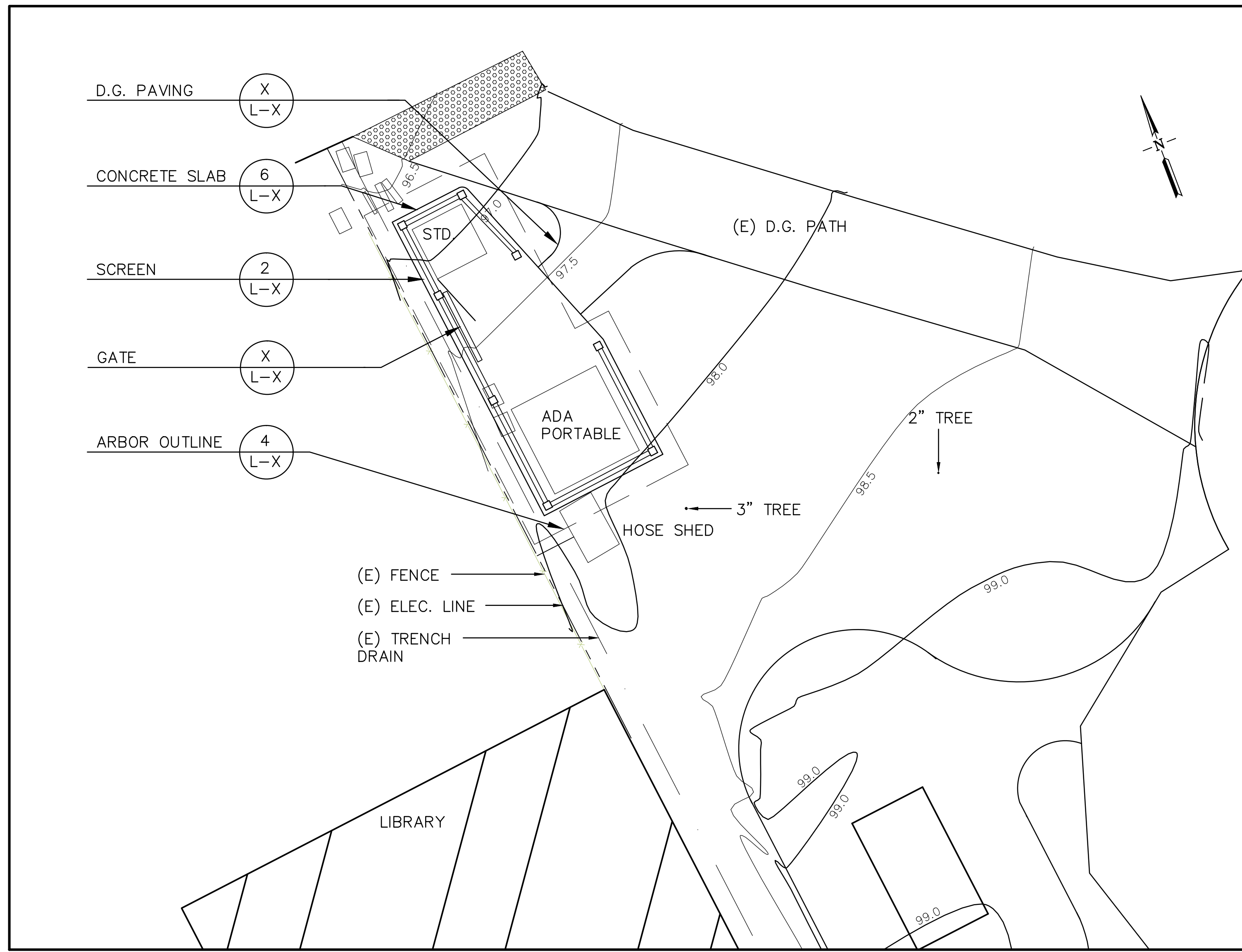
LAYOUT PLAN 1"=5'-0"
